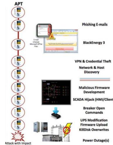
Kill Chain Mapping (SANS)
