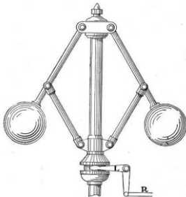
Flyball Governor Mechanical
